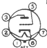
BOTTOM VIEW (G-60)
